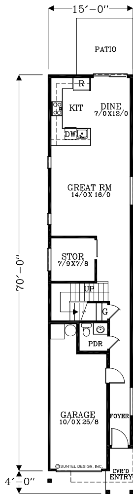
MAIN FLOOR PLAN 791 SQUARE FEET 1,807 TOTAL SQUARE FEET
