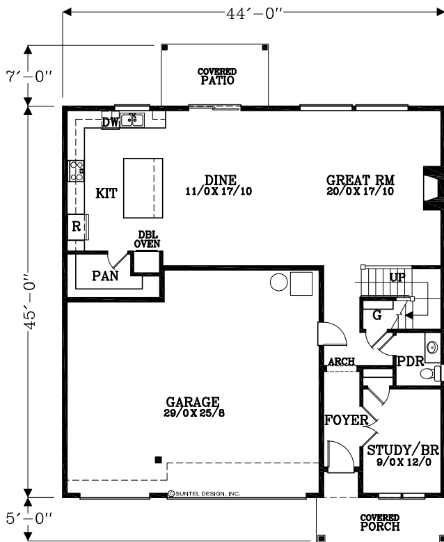
MAIN FLOOR PLAN 1,237 SQUARE FEET 3,048 TOTAL SQUARE FEET
