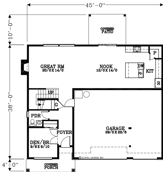
MAIN FLOOR PLAN 1,011 SQUARE FEET 2,465 TOTAL SQUARE FEET
