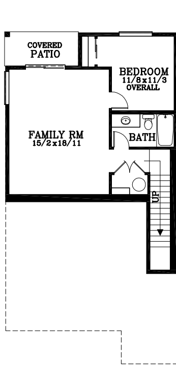
LOWER FLOOR PLAN 560 SQUARE FEET
