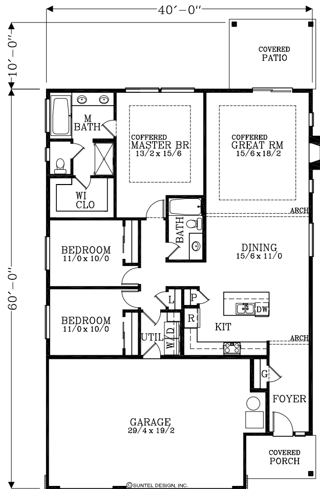
FLOOR PLAN 1,722 TOTAL SQUARE FEET
