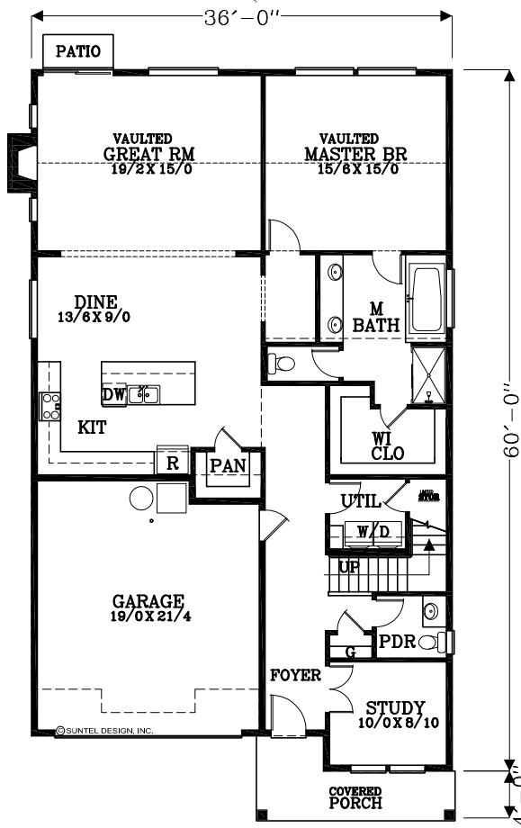
MAIN FLOOR PLAN 1,671 SQUARE FEET 2,583 TOTAL SQUARE FEET
