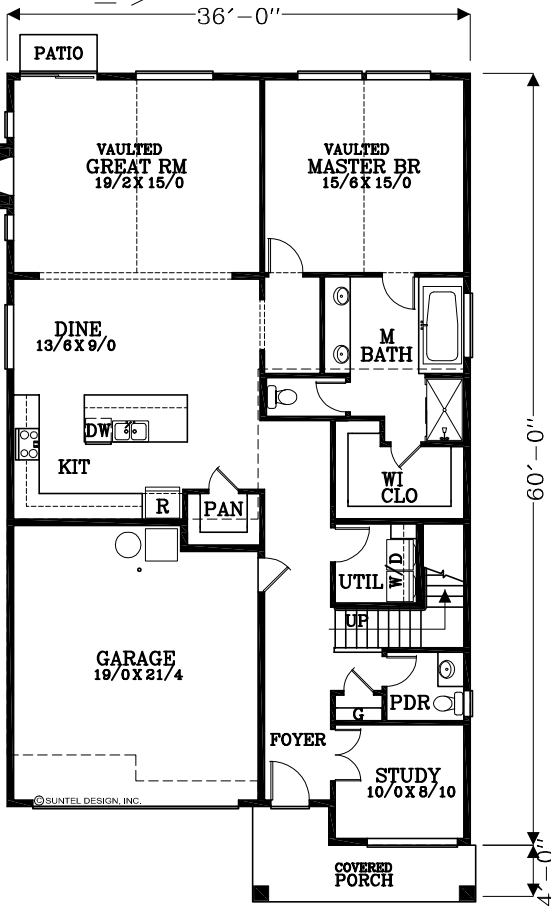
MAIN FLOOR PLAN 1,671 SQUARE FEET 2,586 TOTAL SQUARE FEET
