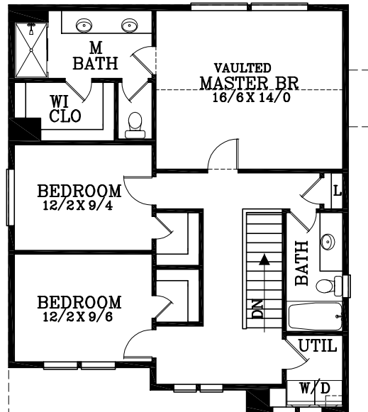
UPPER FLOOR PLAN 981 SQUARE FEET
