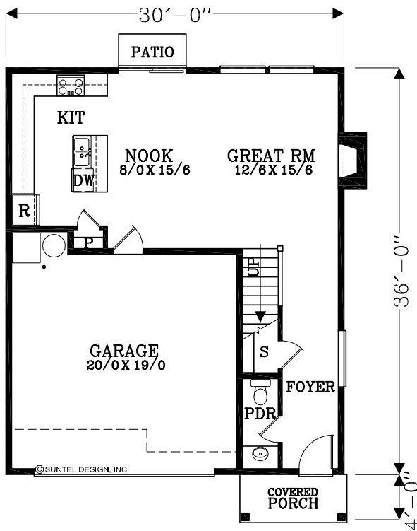
MAIN FLOOR PLAN 669 SQUARE FEET 1,650 TOTAL SQUARE FEET
