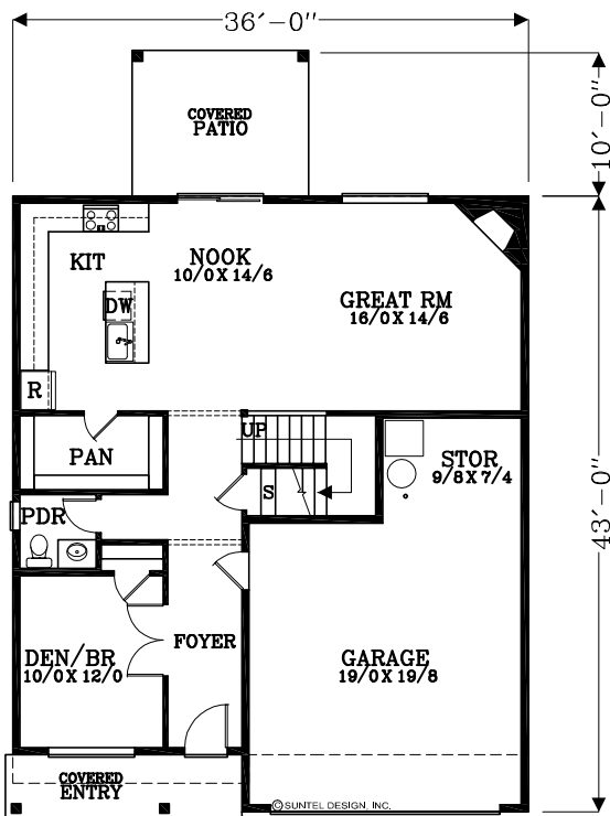
MAIN FLOOR PLAN 1,014 SQUARE FEET 2,383 TOTAL SQUARE FEET
