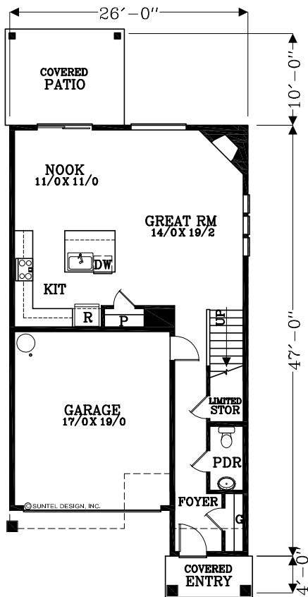
MAIN FLOOR PLAN 793 SQUARE FEET 1,860 TOTAL SQUARE FEET
