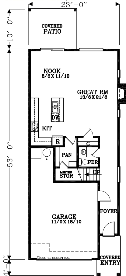
MAIN FLOOR PLAN 792 SQUARE FEET 1,878 TOTAL SQUARE FEET
