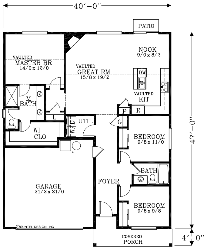
FLOOR PLAN 1,431 TOTAL SQUARE FEET
