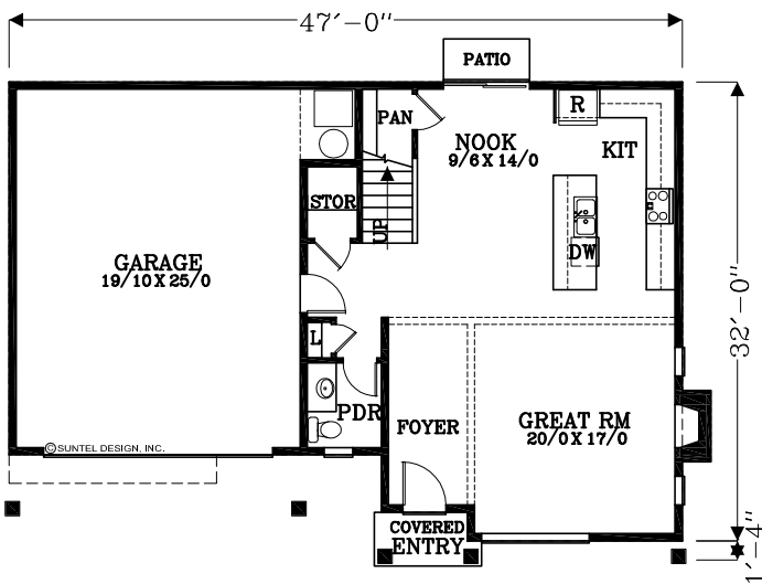
MAIN FLOOR PLAN 787 SQUARE FEET 2,082 TOTAL SQUARE FEET
