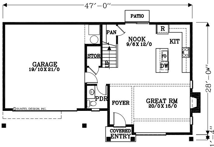
MAIN FLOOR PLAN 700 SQUARE FEET 1,807 TOTAL SQUARE FEET
