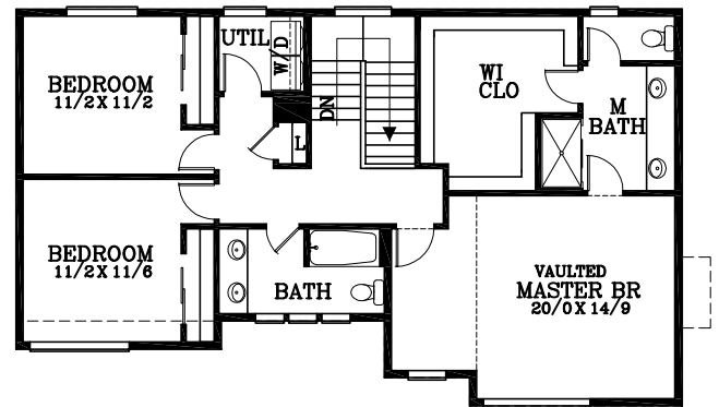
UPPER FLOOR PLAN 1,107 SQUARE FEET
