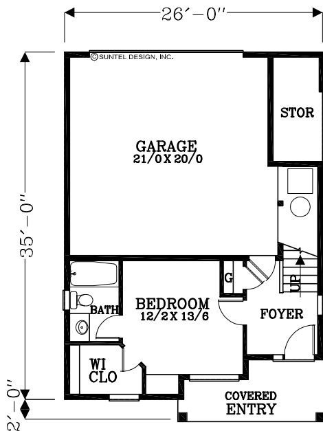
LOWER FLOOR PLAN 376 SQUARE FEET
