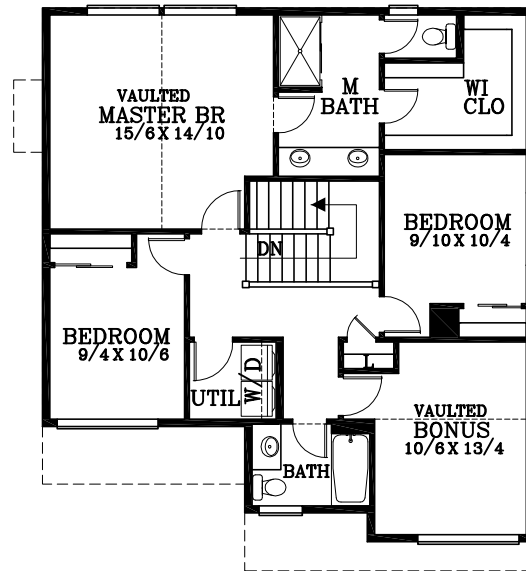
UPPER FLOOR PLAN 1,061 SQUARE FEET
