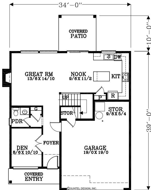
MAIN FLOOR PLAN 807 SQUARE FEET 1,868 TOTAL SQUARE FEET
