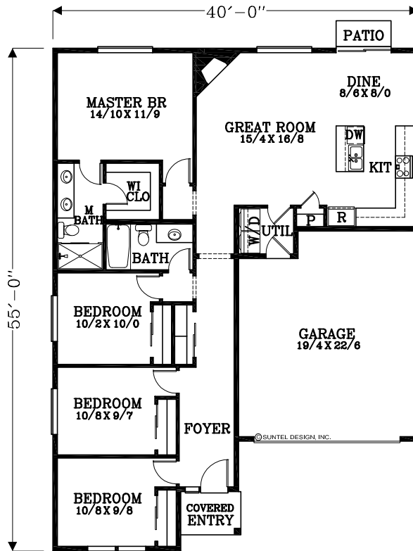
FLOOR PLAN 1,490 TOTAL SQUARE FEET
