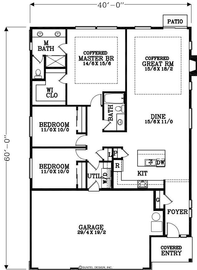
FLOOR PLAN 1,722 TOTAL SQUARE FEET
