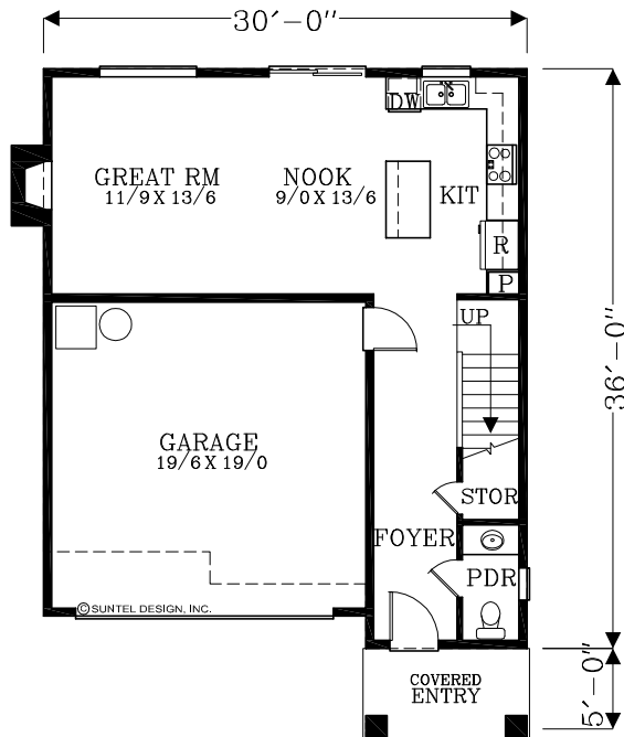
MAIN FLOOR PLAN 630 SQUARE FEET 1555 TOTAL SQUARE FEET
