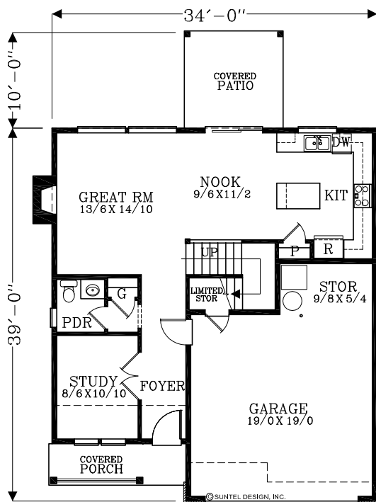
MAIN FLOOR PLAN 807 SQUARE FEET 1868 TOTAL SQUARE FEET
