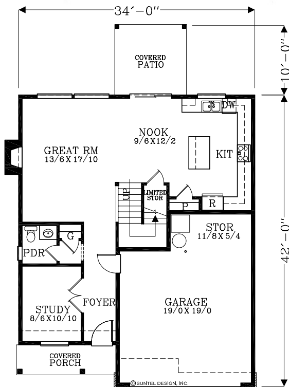
MAIN FLOOR PLAN 895 SQUARE FEET 2,088 TOTAL SQUARE FEET
