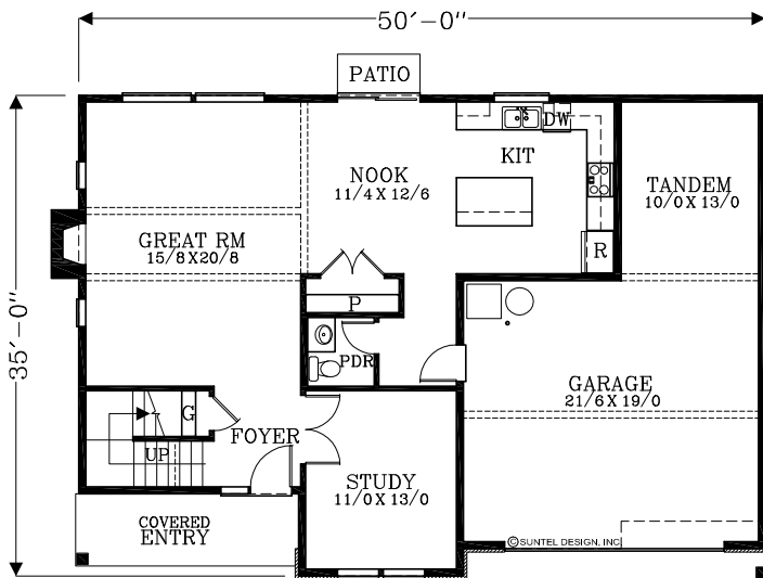
MAIN FLOOR PLAN 1,039 SQUARE FEET 2,566 TOTAL SQUARE FEET
