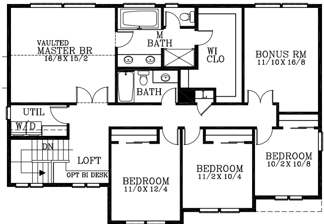
UPPER FLOOR PLAN 1,527 SQUARE FEET
