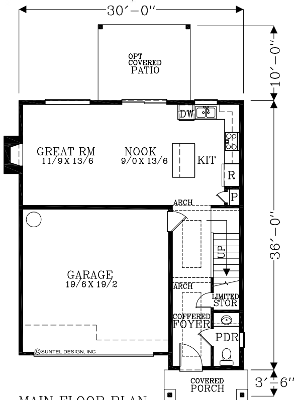
MAIN FLOOR PLAN 630 SQUARE FEET 1555 TOTAL SQUARE FEET
