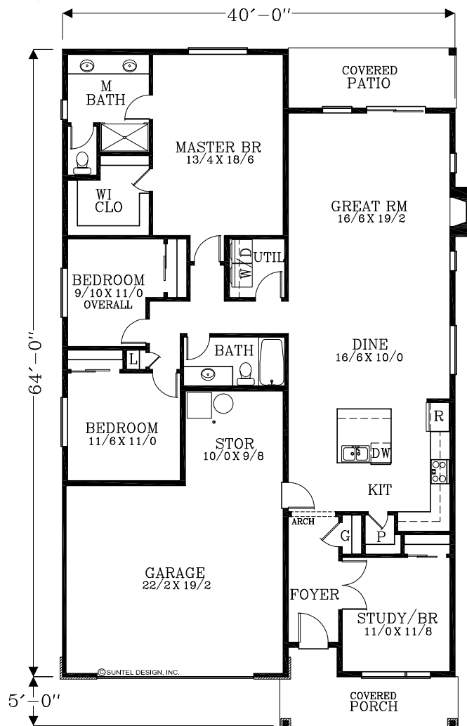
FLOOR PLAN 1,906 TOTAL SQUARE FEET
