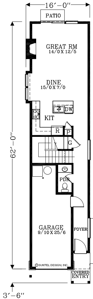
MAIN FLOOR PLAN 679 SQUARE FEET 1561 TOTAL SQUARE FEET
