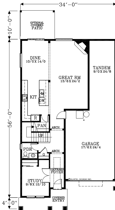
MAIN FLOOR PLAN 843 SQUARE FEET 2825 TOTAL SQUARE FEET
