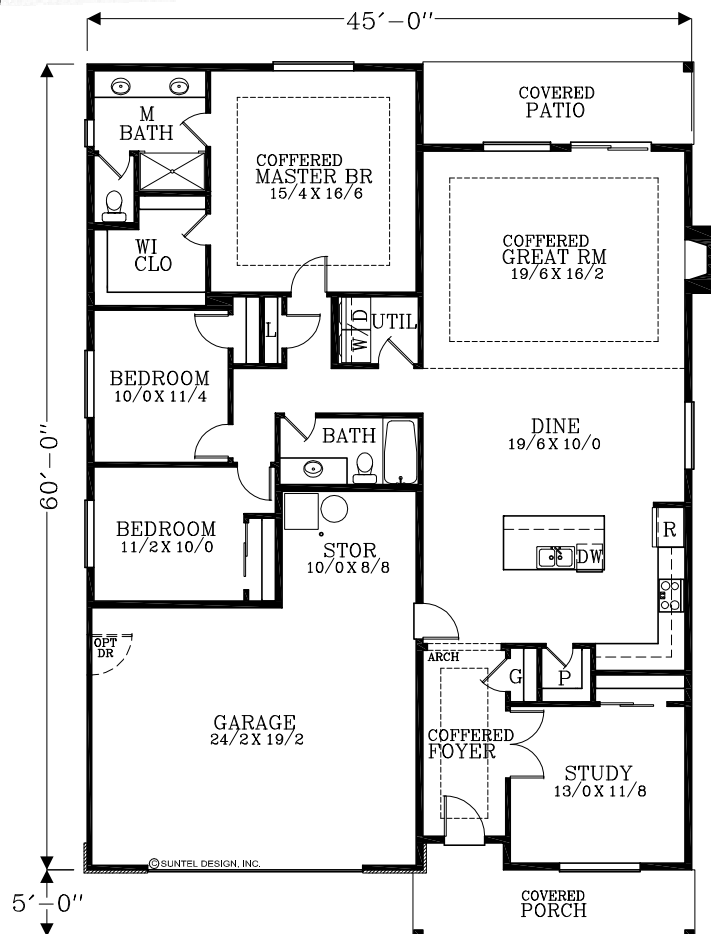
FLOOR PLAN 2,002 TOTAL SQUARE FEET
