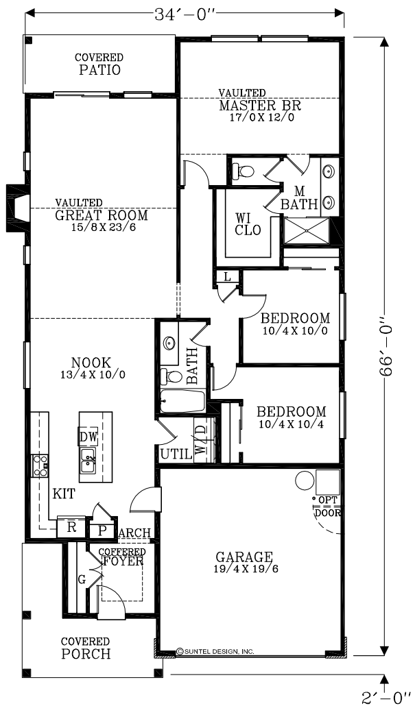
FLOOR PLAN 1665 TOTAL SQUARE FEET
