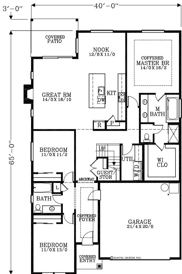
MAIN FLOOR PLAN 1934 SQUARE FEET 2440 TOTAL SQUARE FEET
