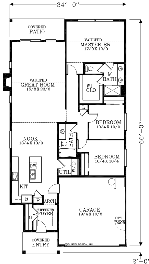
FLOOR PLAN 1665 TOTAL SQUARE FEET
