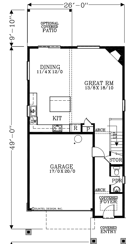
3'-6" MAIN FLOOR PLAN 783 SQUARE FEET 1953 TOTAL SQUARE FEET
