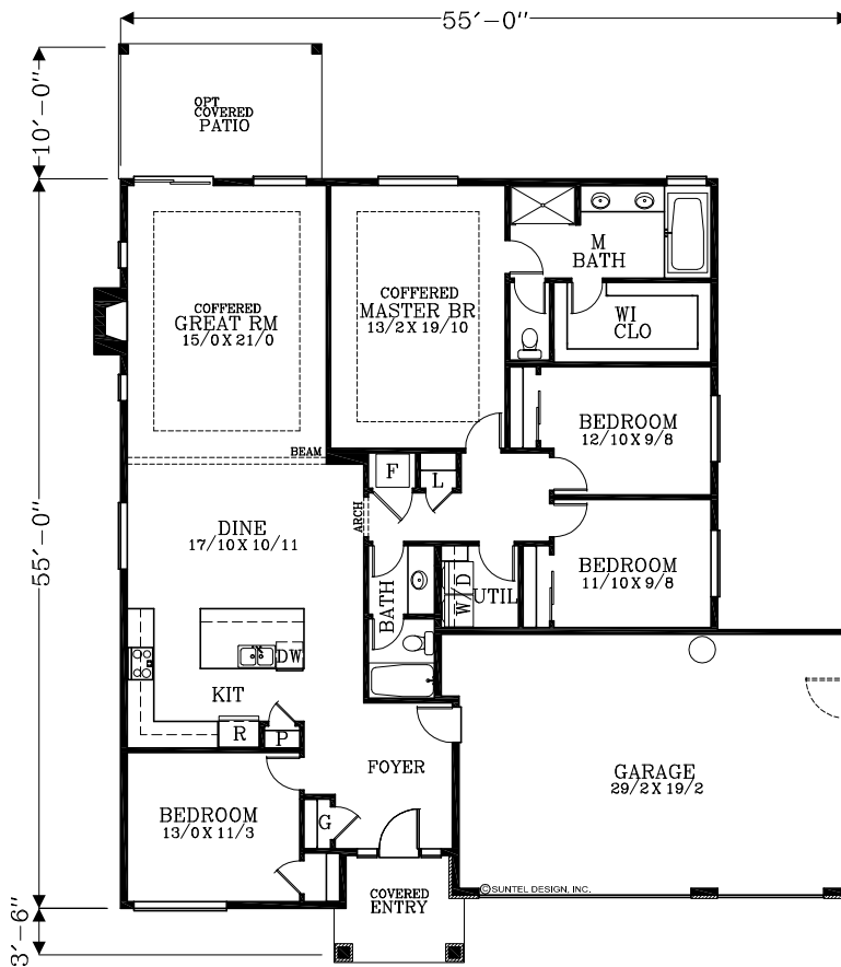
FLOOR PLAN 2,031 TOTAL SQUARE FEET
