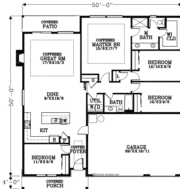
FLOOR PLAN 1826 TOTAL SQUARE FEET
