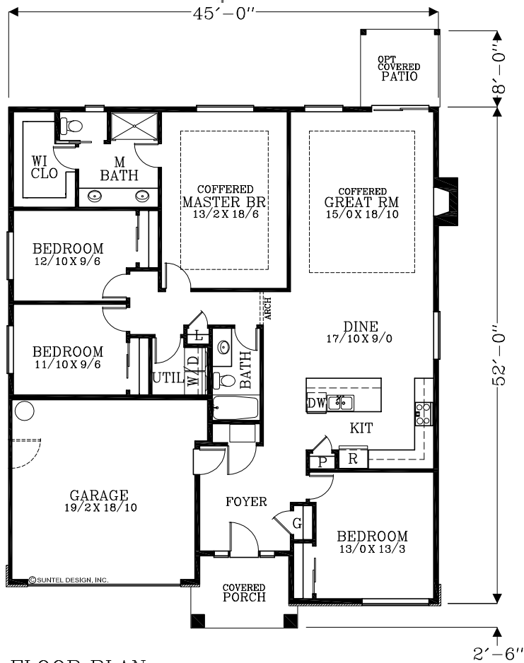
FLOOR PLAN 1,844 TOTAL SQUARE FEET
