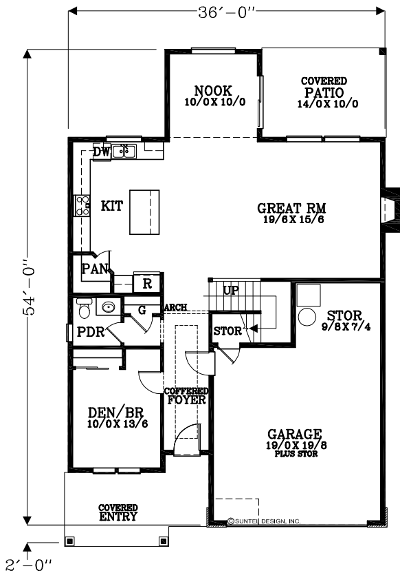
MAIN FLOOR PLAN 1116 SQUARE FEET 2508 TOTAL SQUARE FEET
