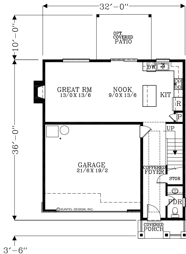
MAIN FLOOR PLAN 658 SQUARE FEET 1635 TOTAL SQUARE FEET
