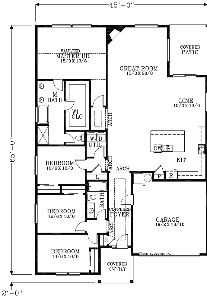
FLOOR PLAN 2248 TOTAL SQUARE FEET
