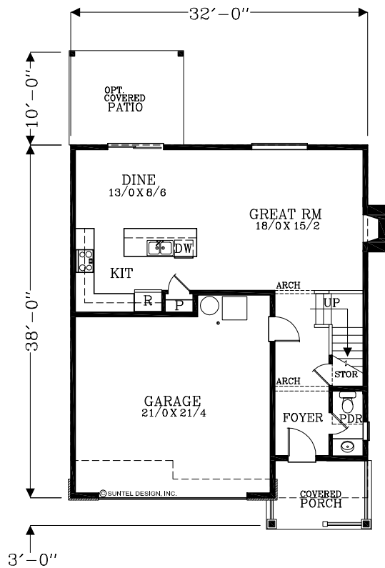
MAIN FLOOR PLAN 736 SQUARE FEET 1848 TOTAL SQUARE FEET
