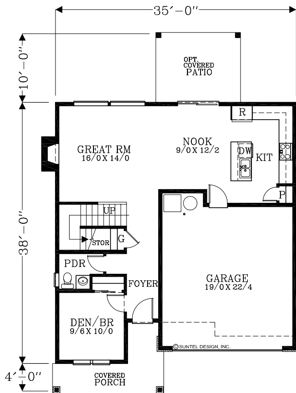
MAIN FLOOR PLAN 843 SQUARE FEET 1886 TOTAL SQUARE FEET
