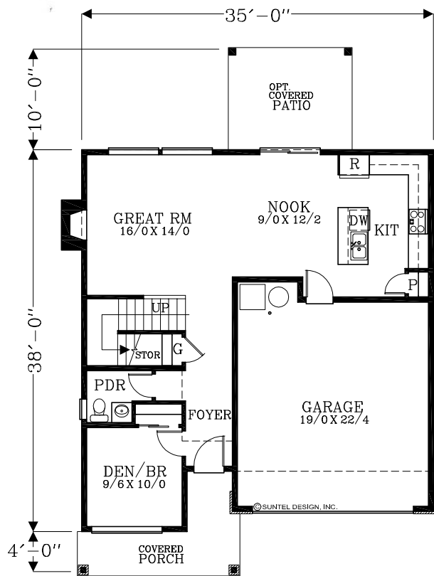
MAIN FLOOR PLAN 843 SQUARE FEET 1786 TOTAL SQUARE FEET
