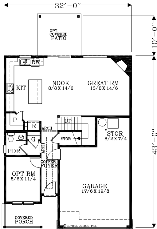
MAIN FLOOR PLAN 856 SQUARE FEET 2031 TOTAL SQUARE FEET
