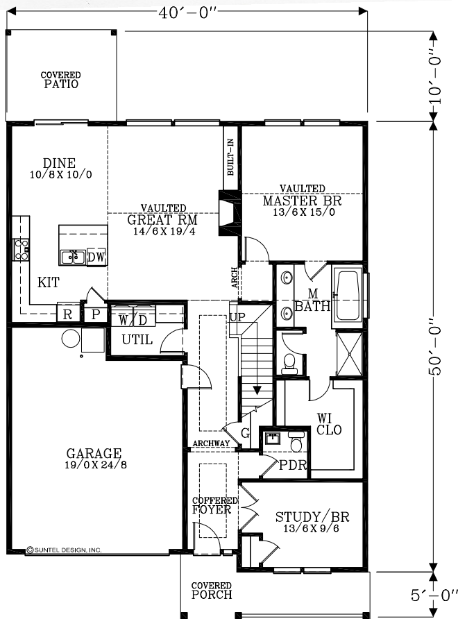
MAIN FLOOR PLAN 1489 SQUARE FEET 2037 TOTAL SQUARE FEET
