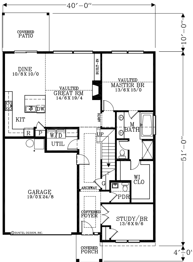
MAIN FLOOR PLAN 1489 SQUARE FEET 2051 TOTAL SQUARE FEET
