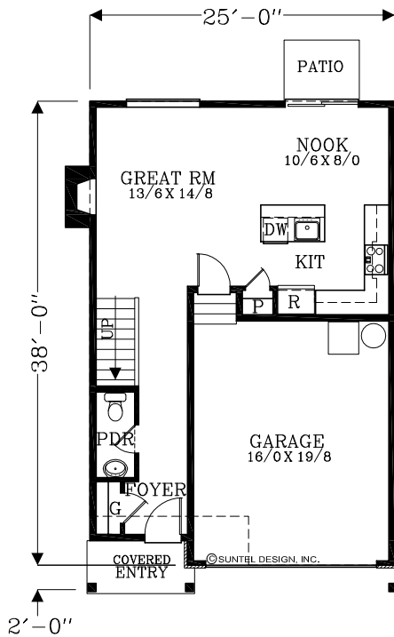
MAIN FLOOR PLAN 595 SQUARE FEET 1455 TOTAL SQUARE FEET
