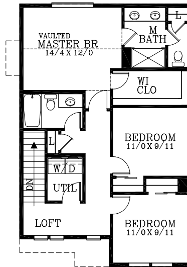
UPPER FLOOR PLAN 860 SQUARE FEET
