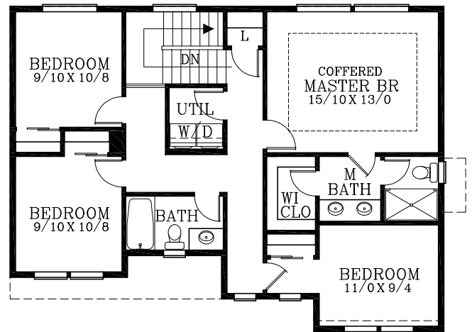
UPPER FLOOR PLAN 994 SQUARE FEET
