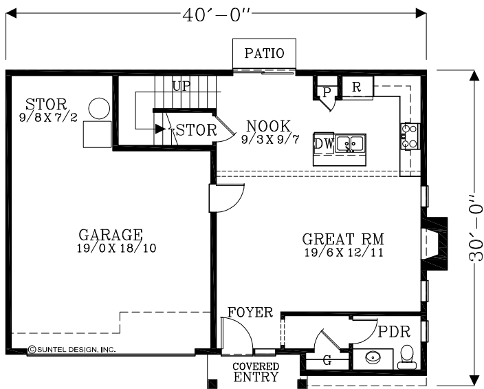
MAIN FLOOR PLAN 649 SQUARE FEET 1643 TOTAL SQUARE FEET
