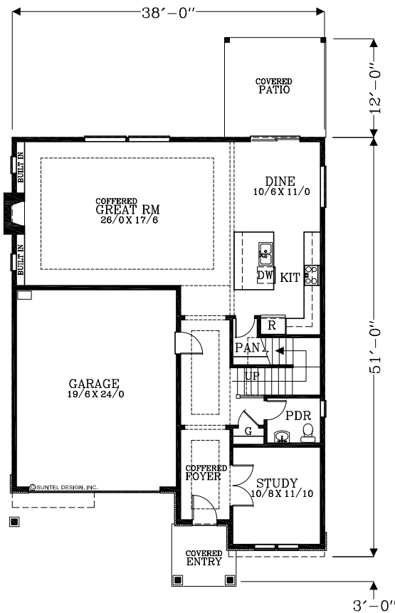
MAIN FLOOR PLAN 1251 SQUARE FEET 2959 TOTAL SQUARE FEET
