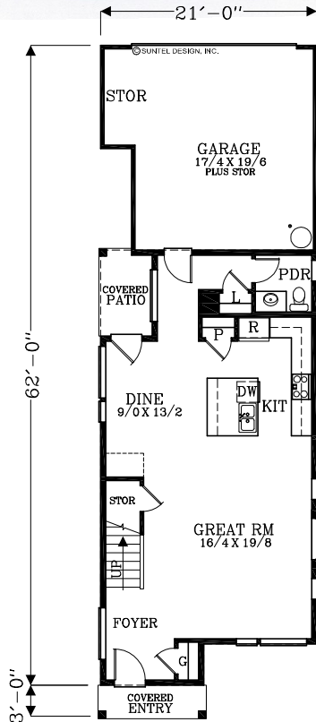
MAIN FLOOR PLAN 800 SQUARE FEET 1602 TOTAL SQUARE FEET
