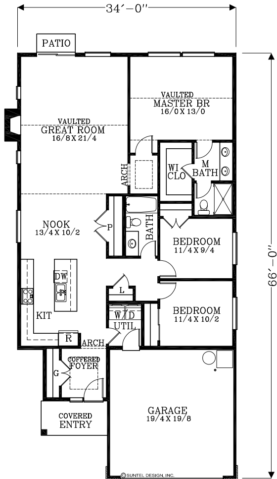
FLOOR PLAN 1649 TOTAL SQUARE FEET
