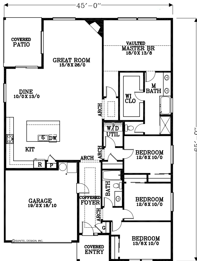
FLOOR PLAN 2248 TOTAL SQUARE FEET
