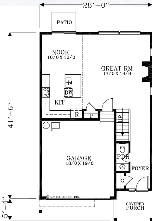
MAIN FLOOR PLAN 774 SQUARE FEET 1909 TOTAL SQUARE FEET
